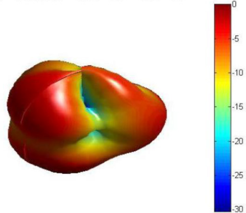
900MHz Freq = 0.9GHz Az= 45 EL= 45
