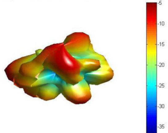
1900MHz Freq = 1.9GHz Az= 45 EL= 45
