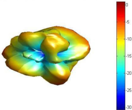
1800MHz Freq = 1.8GHz Az= 45 EL= 45
